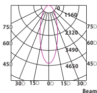
Beam Angle=40°
