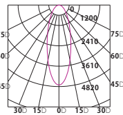
Beam Angle=40°
