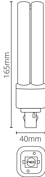
G24D Base lamp
