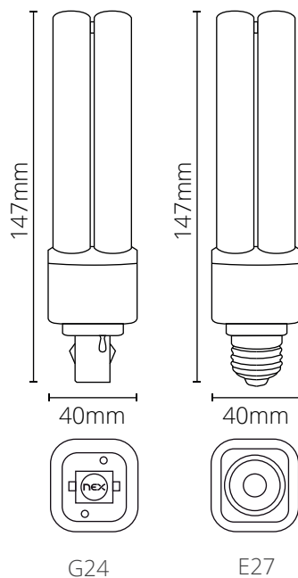
Base lamp
