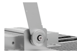
Bracket Cold-rolled steel sheet (SPCC), powder spraying process used on the surface, 3 mm thick
